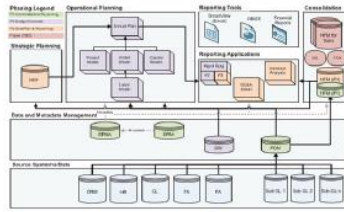
Solution Architecture/Roadmap
